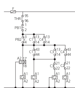
Connection Diagram 2 (HGC115 - 800)
