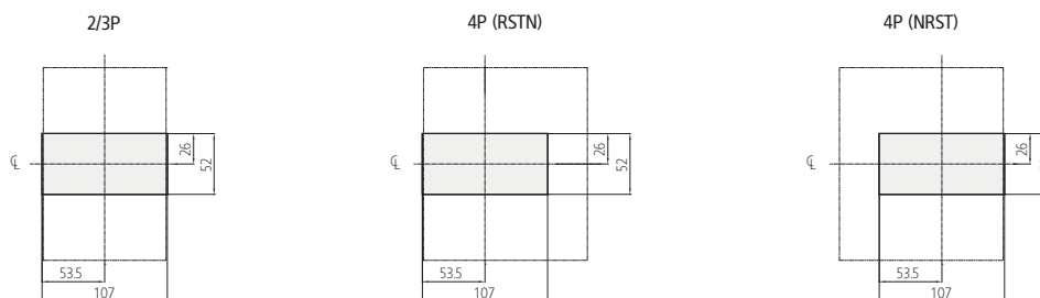
Panel Cover Cutting Dimensions for Handle/Test Button
