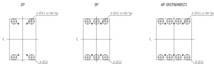
Dimensions for Mounting Body
