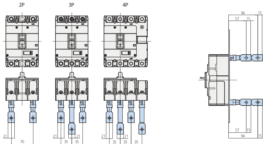
Dimensions for Mounting Body
